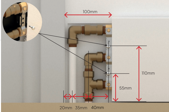
Clockwise Non TRV (For anti-clockwise, (Mirror image).
